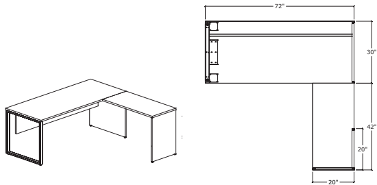
SIMPLICITY TYPICAL #19 • O LEG MODESTY DESK & OPEN RETURN
