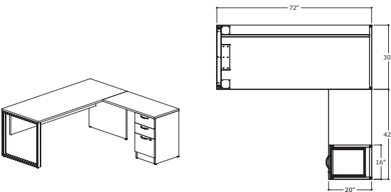
SIMPLICITY TYPICAL #20 • O LEG MODESTY DESK & BOX / BOX / FILE RETURN
