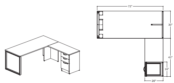
SIMPLICITY TYPICAL #24 • O LEG T GABLE DESK & BOX / BOX / FILE RETURN
