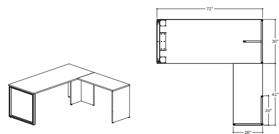
SIMPLICITY TYPICAL #23 • O LEG T GABLE DESK & OPEN RETURN
