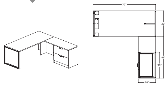
SIMPLICITY TYPICAL #26 • O LEG T GABLE DESK & LATERAL FILE RETURN
